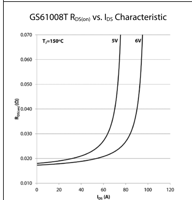
Figure 4: R_{DS(on)} vs. I_{DS} at T_J = 150\text{ }^\circ\text{C}
