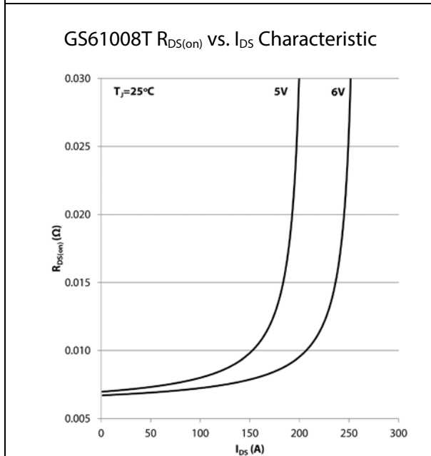
Figure 3: R_{DS(on)} vs. I_{DS} at T_J = 25\text{ }^\circ\text{C}
